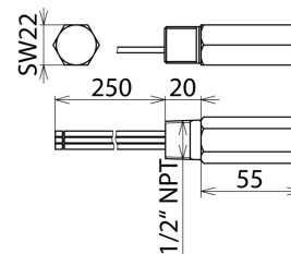
Dimension drawing DPI CD EXI 24 N
