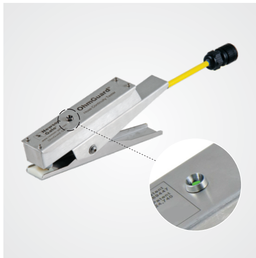
OhmGuard Intrinsically Safe Electrical Continuity Tester
