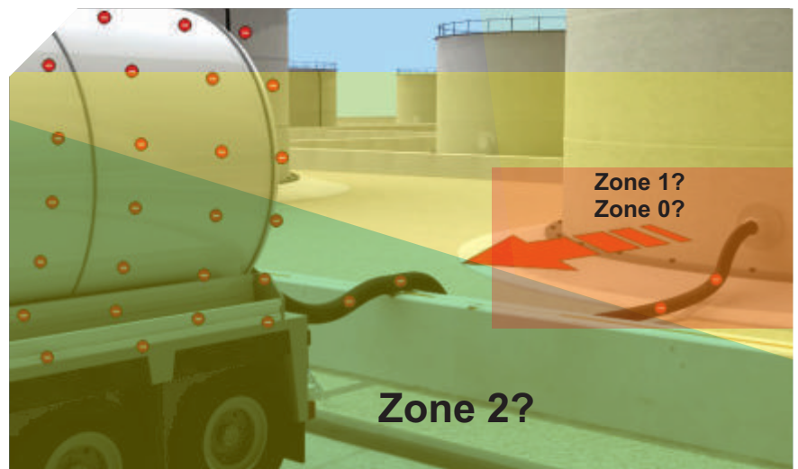
Fig. 4: Vacuum trucks operate in a multitude of environments ranging from Zone 0 areas right through to non-hazardous areas. Providing the right layers of protection from an electrostatic spark can be a significant challenge.
